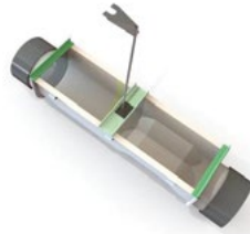
Palmer-Bowlus flumes
